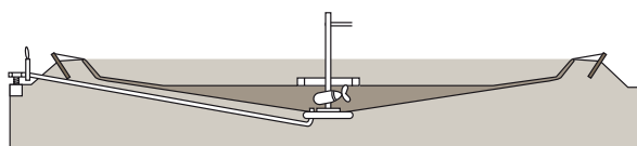
Coupe Alligator Bagtank vide.
